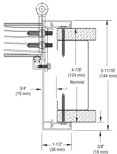
⑥ Strike Jamb with Sidelite/Transom
